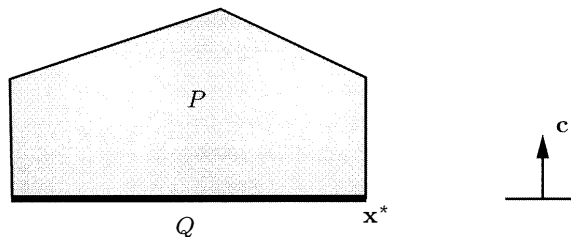
Figure 2.15: Illustration of the proof of Theorem 2.7. Here, Q is the set of optimal solutions and an extreme point \mathbf{x}^* of Q is also an extreme point of P .
