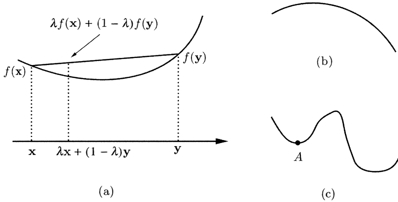
Figure 1.1: (a) Illustration of the definition of a convex function. (b) A concave function. (c) A function that is neither convex nor concave; note that A is a local, but not global, minimum.
